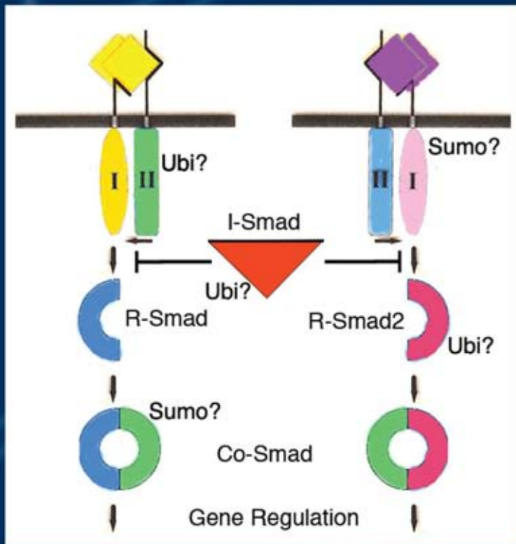
Phylogenetics of TGFβ
